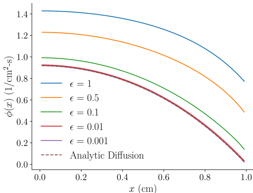
Figure 6: The VEF scalar flux profiles for a range of \epsilon values compared to the exact diffusion solution.
